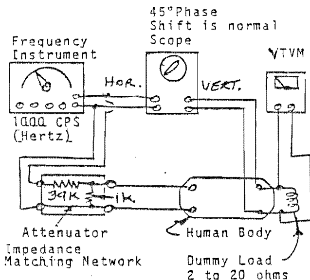
TYPICAL SCOPE-GENERATOR SETUP FOR SIGNAL INPUT/OUTPUT COMPARISON
